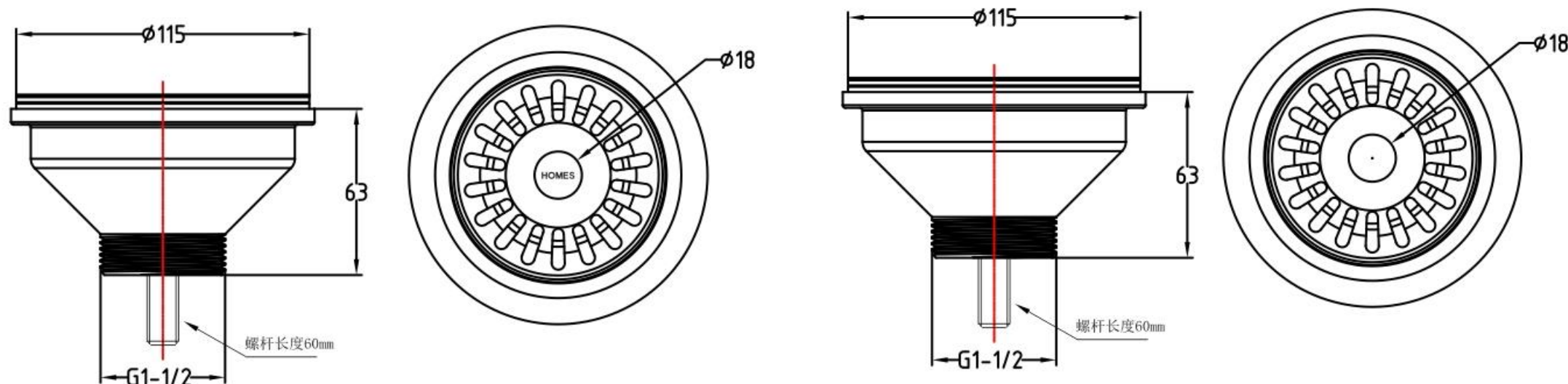
Model: WE313C 传统陶瓷塞头厨房下水过滤篮 Traditional Basket Strainer Waste with Ceramic Plug
