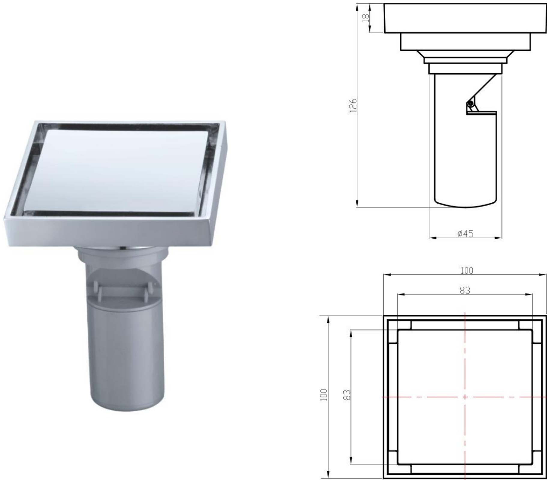
Model: WE501 100x100mm四方铜磁悬浮防臭地漏 100x100mm Brass Square Anti Odormagnetic Suction Technology Floor Drain
